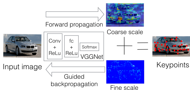
Fig. 1. Overview of weakly supervised keypoint detection pipeline. The input image is fed to a pretrained network on classification, with an occluder to obtain the coarse scale heatmap, and then guided backpropagation is performed to get the fine scale heatmap. The results are combined to produce the log-likelihood distribution for keypoints.
